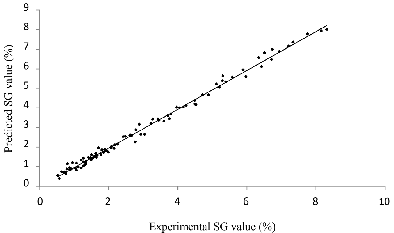
Figure 4. Experimental vs. predicted values for solid gain of osmotically dehydrated potato by optimum GA-NN configuration (R = 0.997).
