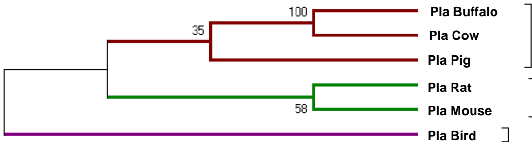
Figure 2(e). Molecular phylogenetic analysis of pla2g XIII gene in different organisms by maximum likelihood method.
