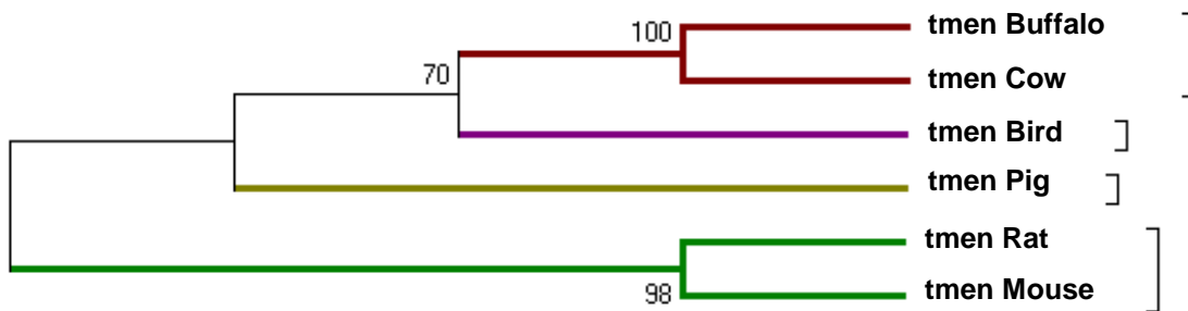
Figure 2(g). Molecular phylogenetic analysis of tmem gene in different organisms by maximum likelihood method.
