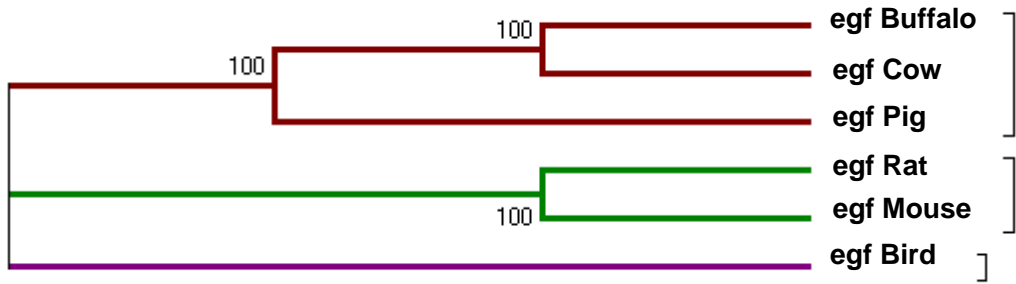
Figure 2(c). Molecular phylogenetic analysis of efg gene in different organisms by maximum likelihood method.
