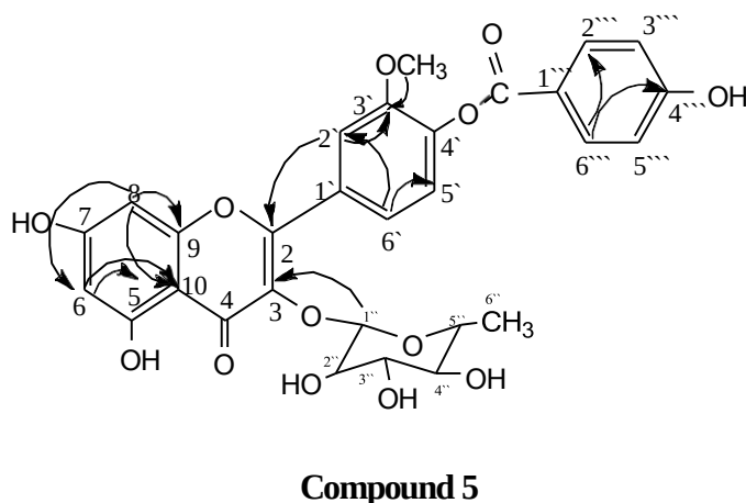
Figure 1. Isolated flavonoids and HMBC correlation of compound 5.
