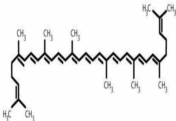
Figure 1. Structural formula of lycopene.
