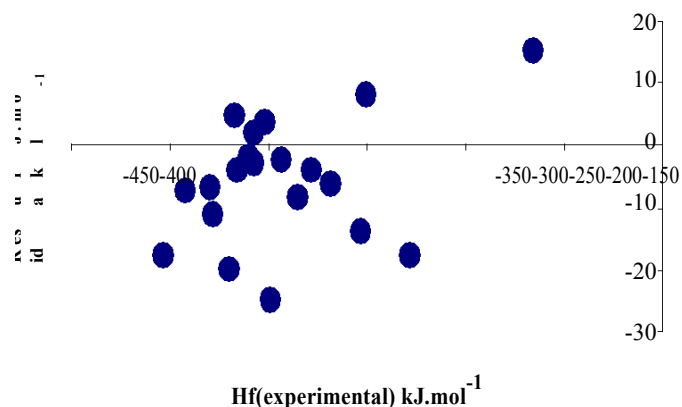
Figure 2. The plot of the residuals versus experimental values error in using MLR model, because of propagation of residuals on the both sides of zero.
