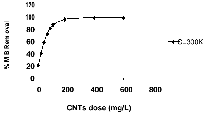
Figure 4. Effect of adsorbent dose on the adsorption percentage of MB onto CNTs.
