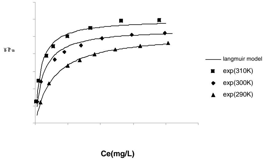
Figure 9. Langmuir isotherm for MB adsorption onto CNTs.
