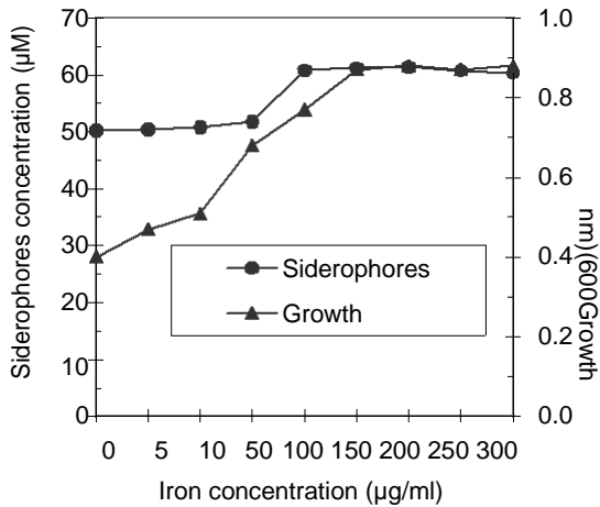
Figure 4. Siderophore production by P. fluorescens P5-18 as a function of Fe (III) added to the succinate medium with 30 units /ml of penicillin.
