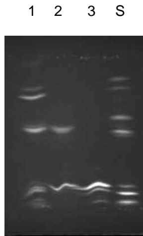
Figure 2. IEF profiles of pyoverdines from P. fluorescens : P1-14 (lane 1), P5-18 (lane 2) and P20-46 (lane 3) with isoelectric pH (pI) internal standards revealed under UV light following electrophoresis (see Meyer et al., 1998).
