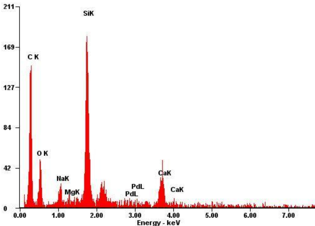
Figure 1. EDX analysis of tea waste biomass.
