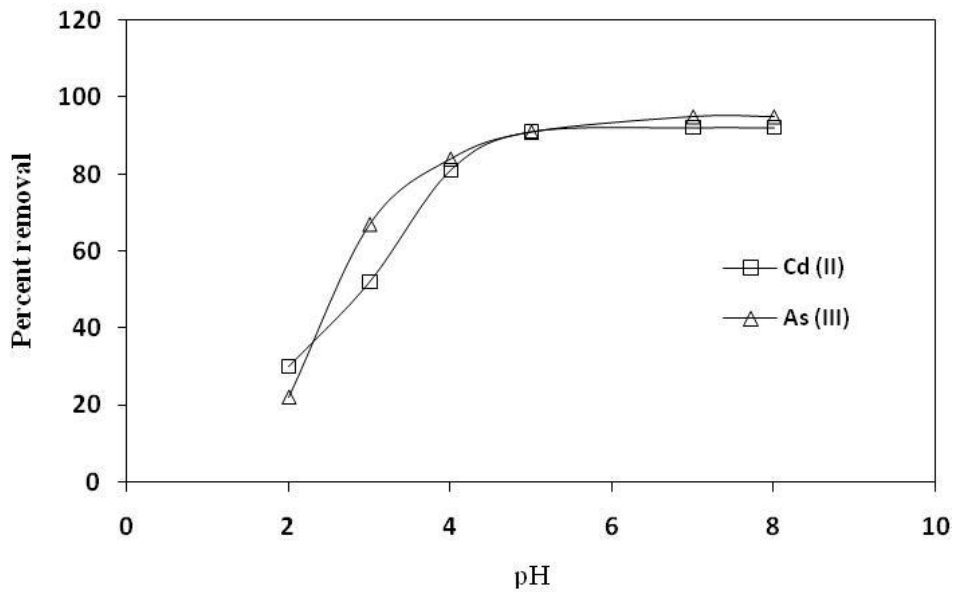
Figure 4. Effect of pH on the biosorption of metal ions onto tea waste biomass.
