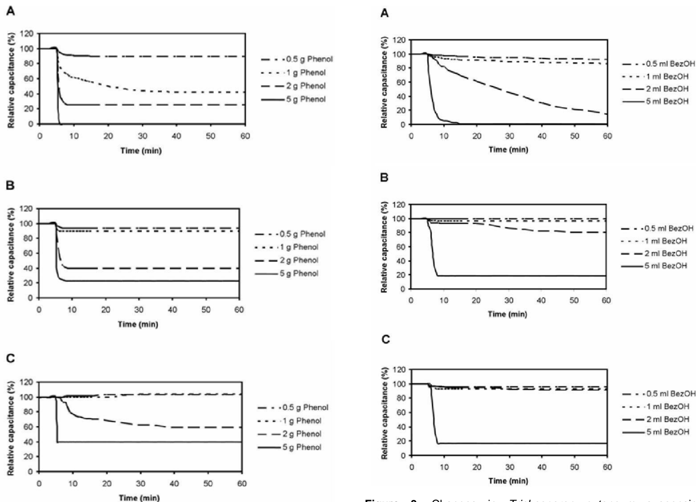
Figure 3. Changes in Trichosporon cutaneum suspension capacitance after the addition of different volumes of benzylalcohol to 100 ml cell suspension. A: Unconditioned cells grown on glucose (2%). B: After conditioning on phenol medium (1 g/L) for the first time. C: After conditioning on phenol medium (1 g/L) for the second time.
