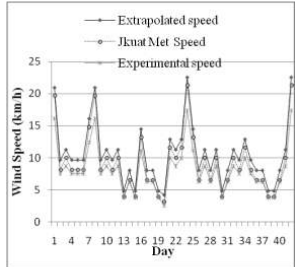
Figure 1. Wind speed profile at 9.00 a.m.
