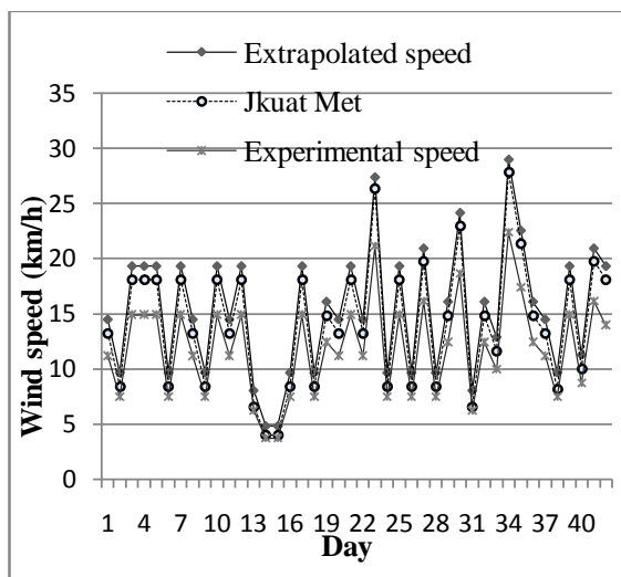
Figure 3. Wind speed profile at 5.00 pm.
