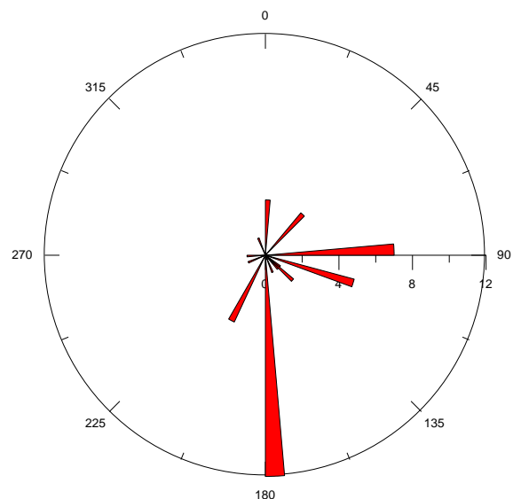
Figure 5. Wind rose for 2 m height at 12.00 noon in Juja.
