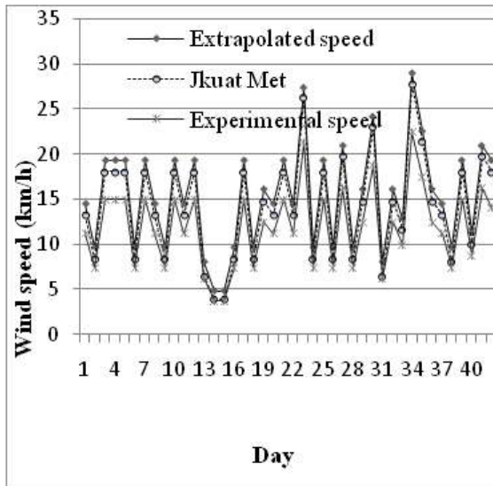
Figure 2. Wind speed profile at 12.00 noon.
