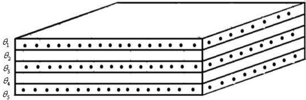
Figure 4. Composite laminate illustrating the design parameters.
