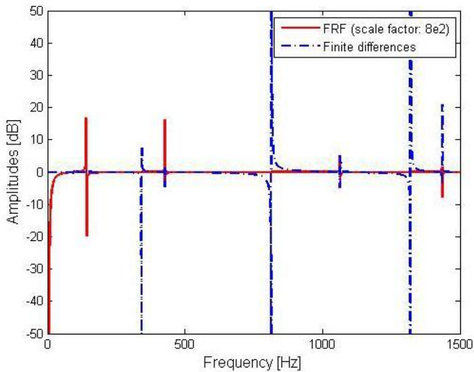
Figure 7. Sensitivity of the FRF obtained with respect to \theta_5 for \theta_5/\theta_5 = 1\% .
