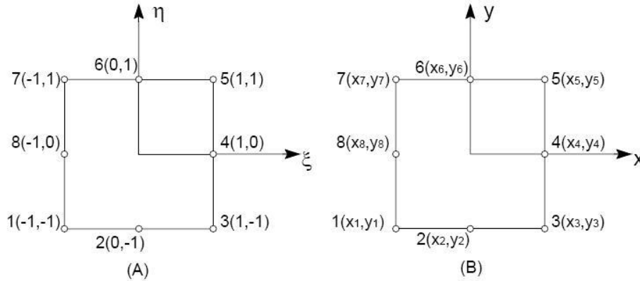
Figure 1. Serendipity family element used in the finite element formulation of laminated composite plates: (a) local coordinates, (b) coordinates.
