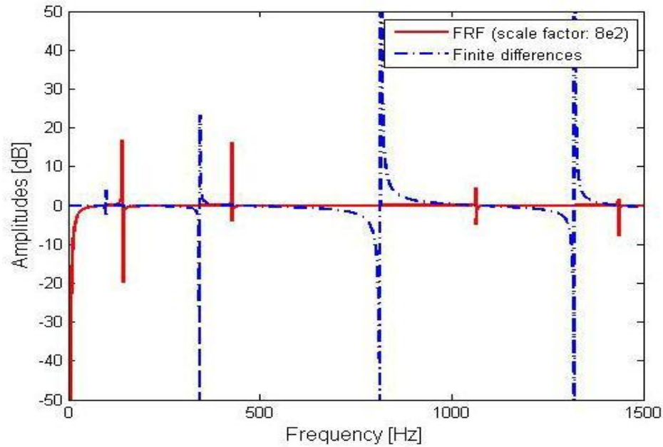
Figure 6. Sensitivity of the FRF obtained with respect to \theta_3 for \theta_3/\theta_3 = 1\% .
