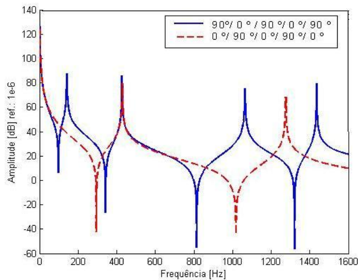
Figure 3. Vibration amplitudes for different stacking sequences.
