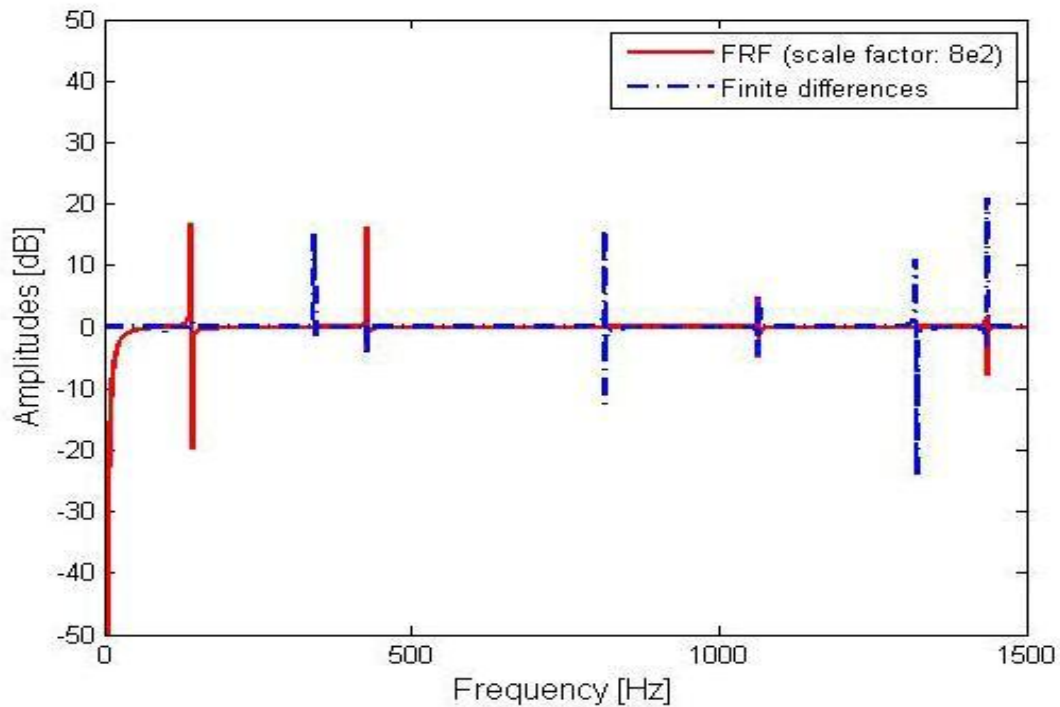
Figure 5. Sensitivity of the FRF obtained with respect to \theta_1 for \Delta\theta_1 = 1\% .
