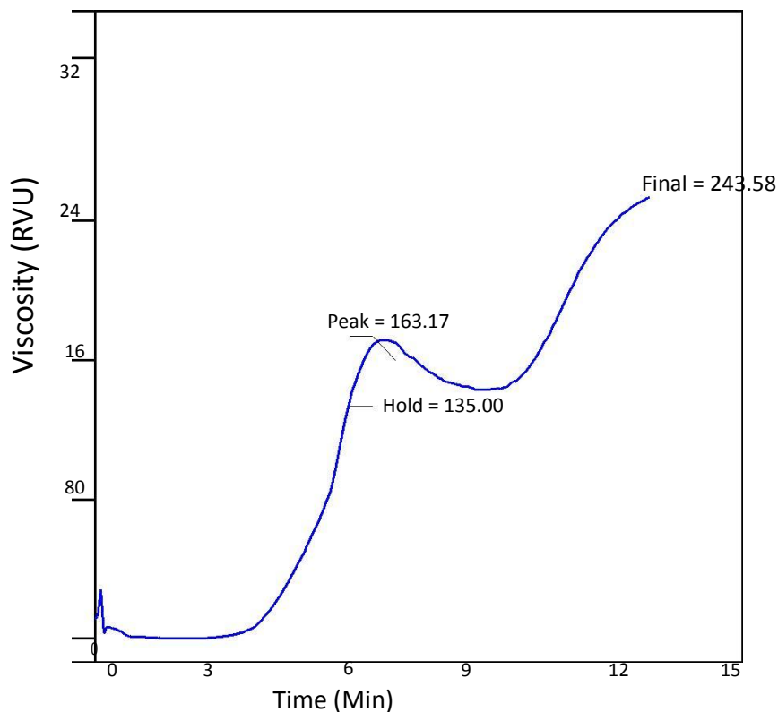
Figure 3. Pasting curve of french horn plantain starch.
