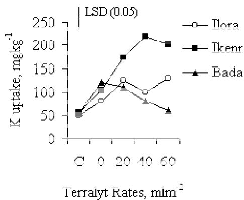
Figure 4. Effect of Terralyt on nutrients uptake of maize.
