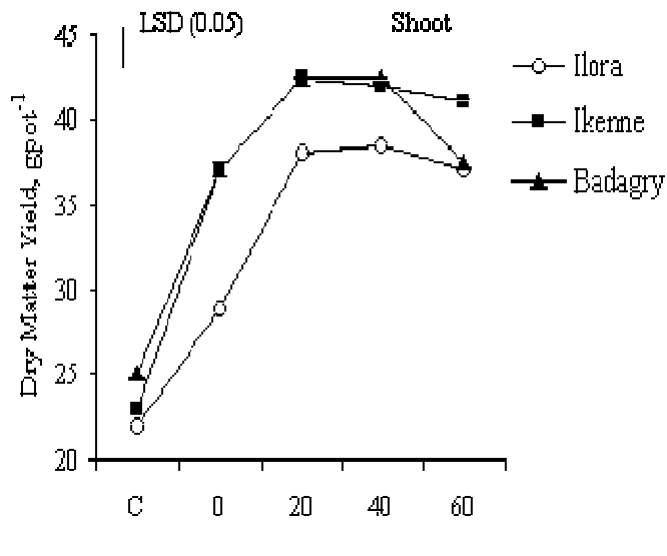
Figure 3. Effect of different rates of Terralyt on dry matter yield of maize.
