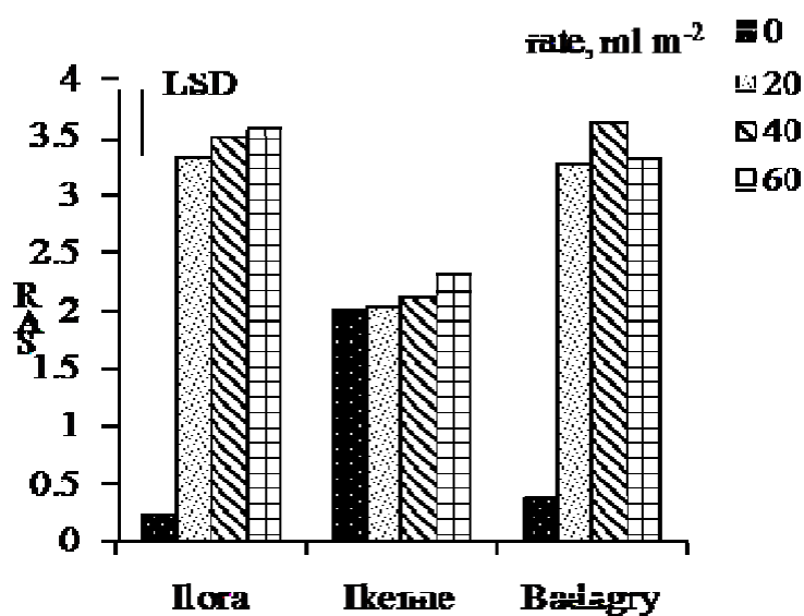
Figure 1. Influence of Terralyt application on soil sodium adsorption ratio (SAR) at post – harvest sampling.
