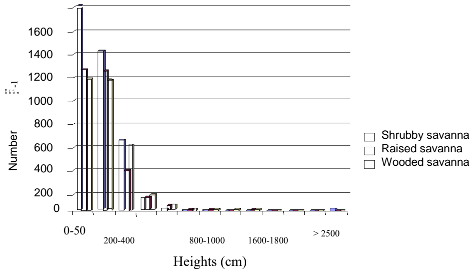
Figure 2. Structure of the population according to the size of the trees.
