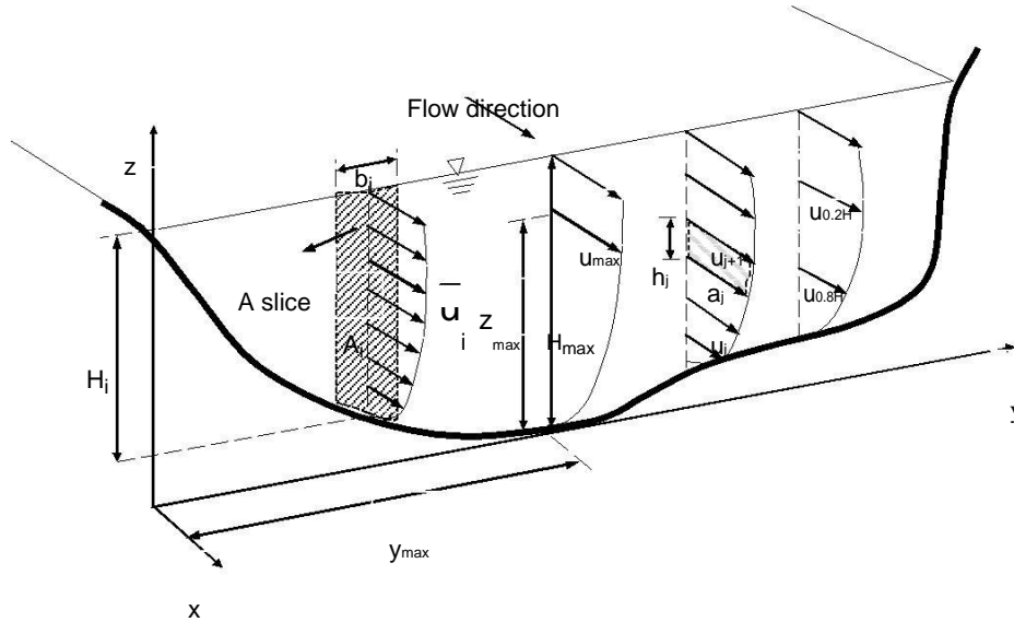
Figure 1. Velocity distribution in measuring cross-section.
