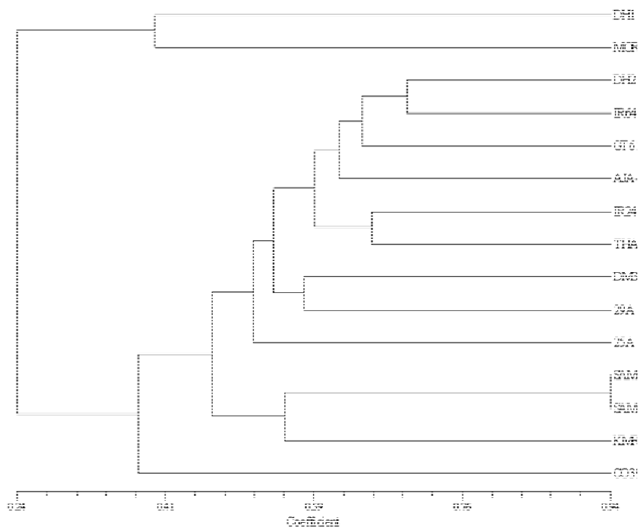
Figure 1. Clustering of 15 O. sativa species based on pooled SSR markers.
