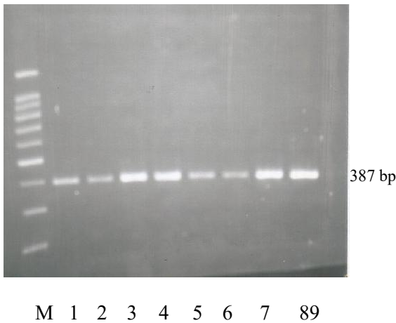
Figure 1. Electrophoretic profiles of PCR products from different storage conditions and temperatures. M = DNA ladder (100 bp), lane 1 = Allantoic fluid (AF) onto filter paper at room temperature, lane 2 = AF onto filter paper at 37°C, lane 3 = AF in liquid at room temperature, lane 4 = AF in liquid at 37°C, lane 5 = Chicken embryo fibroblast (CEF) cell culture onto filter paper at room temperature, lane 6 = CEF cell culture onto filter paper at 37°C, lane 7 = CEF cell culture supernatant at room temperature, lane 8 = CEF cell culture supernatant at 37°C, lane 9 = negative control.
