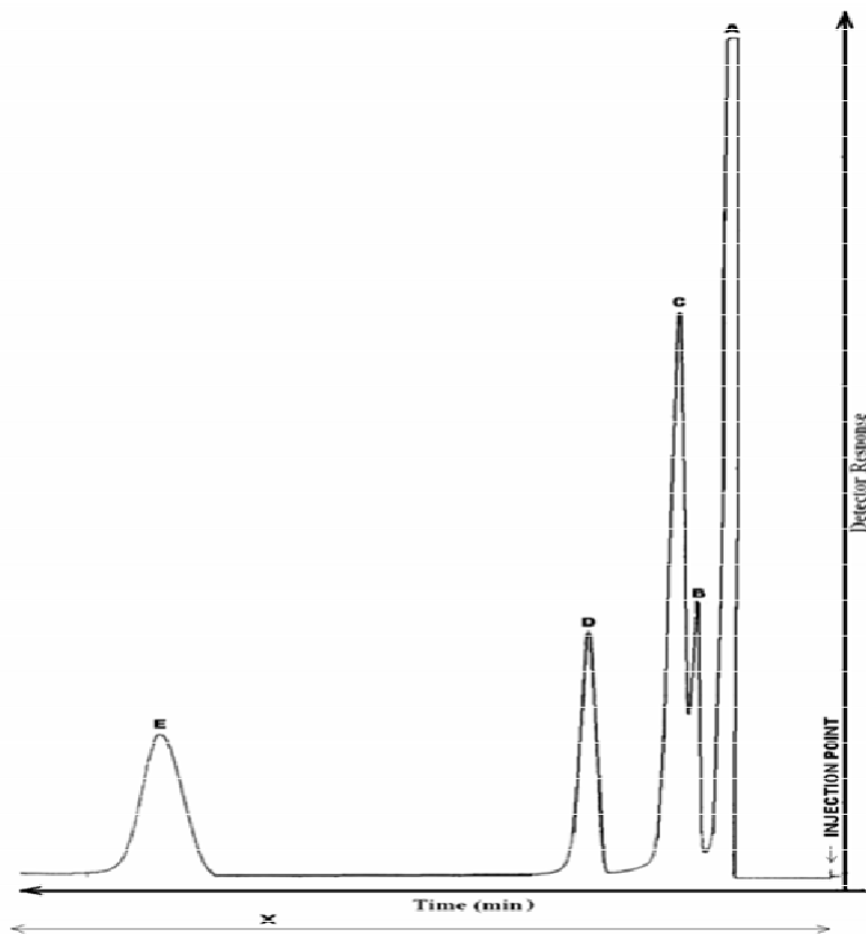
Figure 1. Alcohol profile of standard alcohol mixture. Attenuation condition: 64 \times 10^2 (100mV x 2). A = Acetone + Isopropanol, B = Methanol, C = Ethanol, D = Isoamyl alcohol and E = Butanol.
