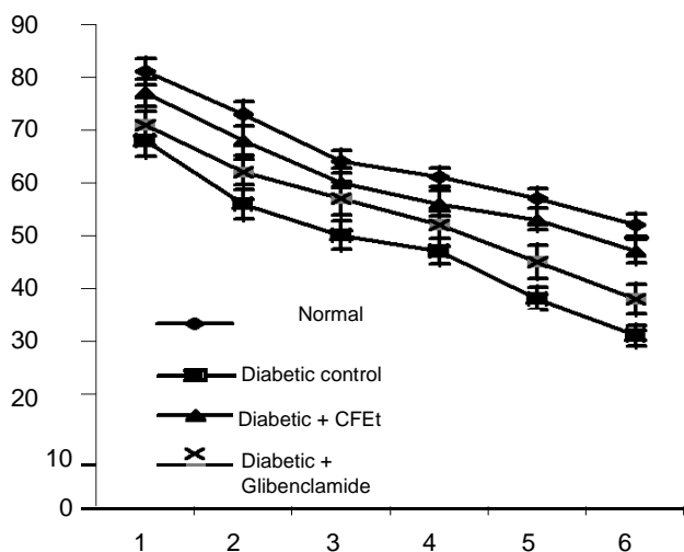
Figure 2. Competitive binding curves showing the effect of CFET and glibenclamide in diabetic rats on the binding of insulin to its receptor on erythrocytes. Percentage of 125 I-insulin bound is plotted as a function of the unlabelled insulin concentration.
