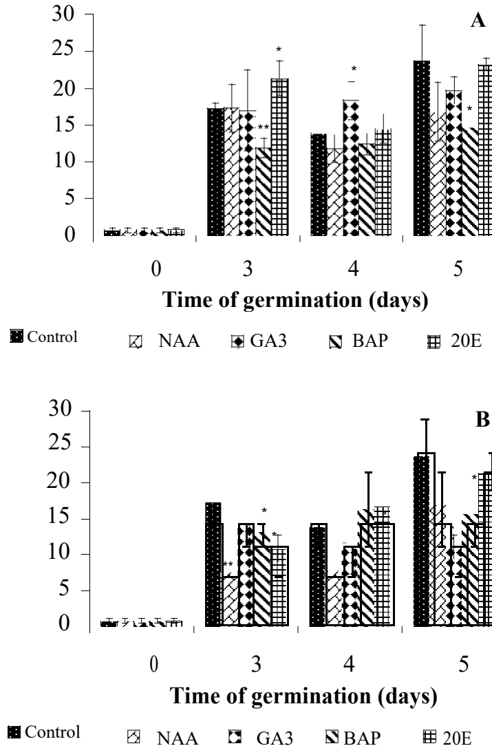
Figure 6. The effect of plant hormones and 20-hydroxyecdysone on proline content in seedlings from germinating tomato seeds. Each value represents the mean + SE of 3 replications. (A): treatment at 10^{-4} M. (B): Treatment at 10^{-5} M. *, ** and *** indicate significant at P 0.05, 0.01 and 0.001 levels, respectively. NAA: acid naftalen acetic; BAP: benzyl amino purine; GA 3 : gibberellic acid ; 20E: 20-hydroxyecdysone.
