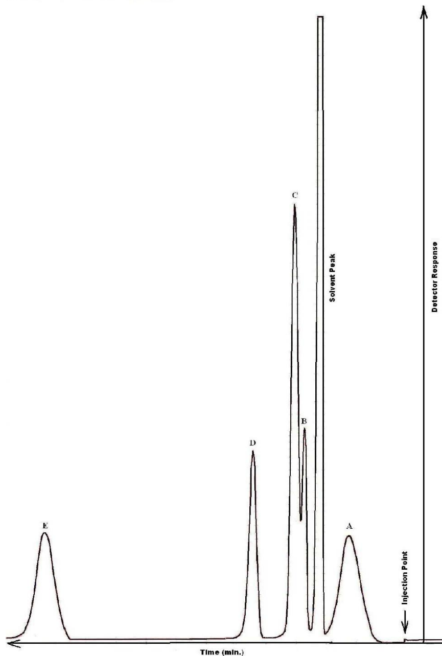
Figure 3. Alcohol profile of standard alcohol mixture. Attenuation condition: 64 \times 10^2 ( 10 \text{ mV} \times 1 ). A = Isopropanol, B = Methanol, C = Ethanol, D = Isoamyl alcohol and E = Butanol
