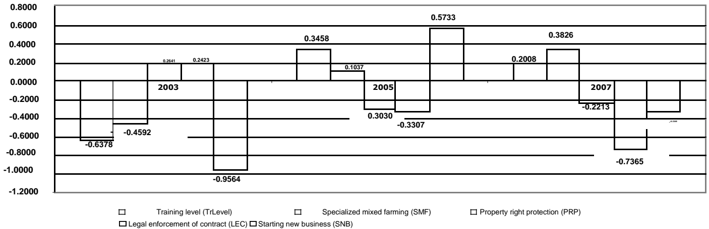
Figure 1. Efficiency determinants patterns (source: Own calculations).
