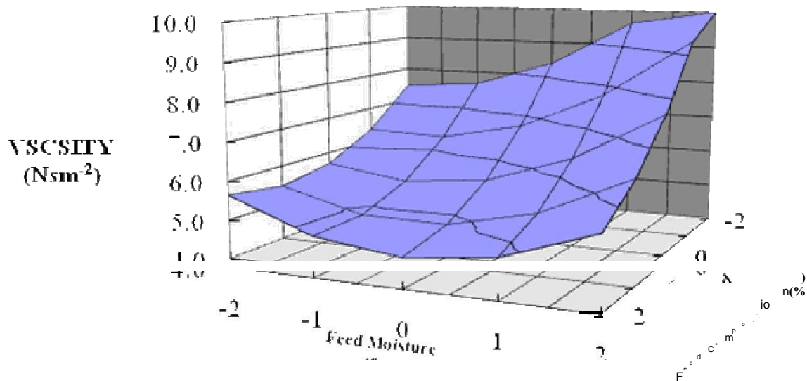
Figure 3. Effect of feed moisture and feed composition on viscosity.
