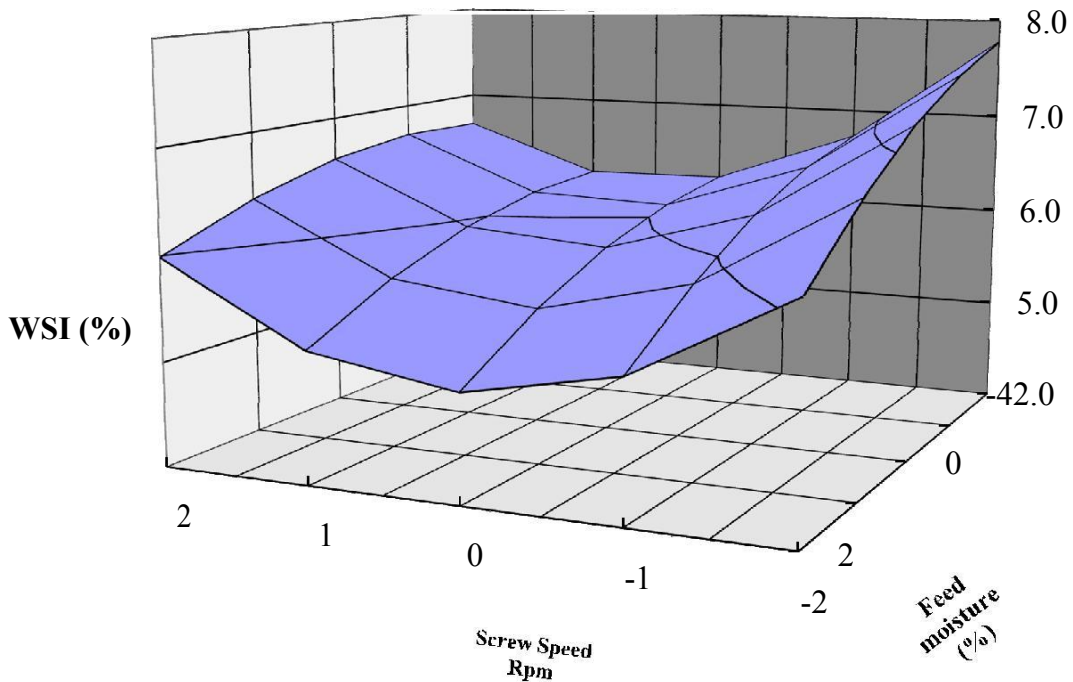
Figure 2. Effect of screw speed and feed moisture on WSI.
