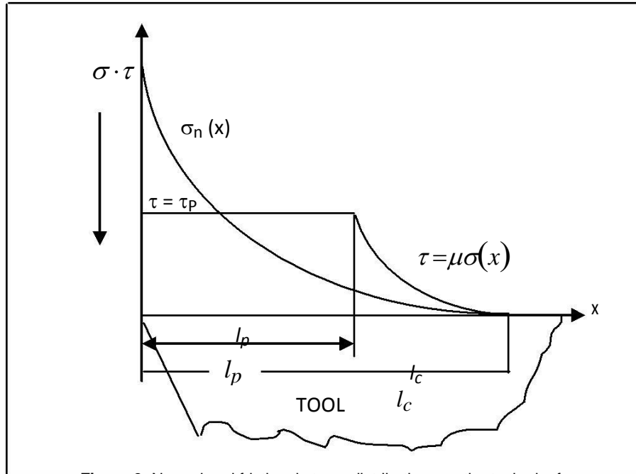
Figure 3. Normal and frictional stress distributions on the tool rake face.
