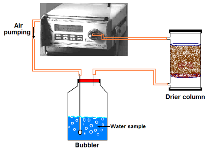
Figure 2. The PRASSI system set up for radon measuring in the water sample.
