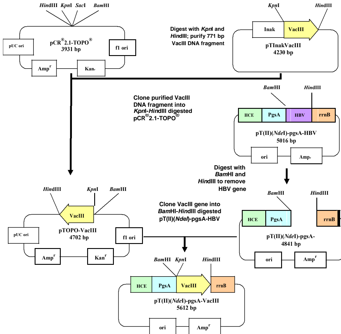
Figure 1. The construction of surface display plasmid pT(II)( NdeI )-pgsA-VacIII which has been used throughout this study. Digestion of pTInakVacIII with KpnI and HindIII restriction enzymes produced two fragments 771 and 3459 bp. The 771 bp (VacIII gene) was ligated with KpnI - HindIII digested pCR ® 2.1-TOPO ® to produce pTOPO-VacIII. Then the pTOPO-VacIII was subjected to Bam HI and HindIII digestion resulted in two fragments of 771 bp (VacIII) and 3.9 kb (pCR ® 2.1-TOPO ® vector). The gel purified VacIII DNA fragment was ligated into Bam HI - HindIII digested pT(II)( NdeI )-pgsA-HBV to generate the surface display plasmid pT(II)( NdeI )-pgsA-VacIII. The plasmid was transformed into S. typhi Ty21a and named as rSTvacIII.
