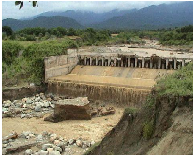
Figure 2. Jafarabad dam - After scouring.
