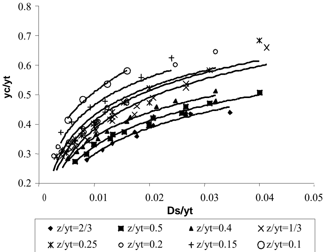
Figure 7. Relation of Ds/yt with z/yc for variable ratio of z/yt ratios.
