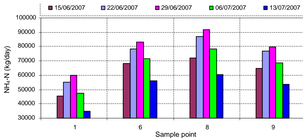
Figure 18. Variation of Ammonium as Nitrogen (NH 4 -N) in kg/day along the Lakhya River.
