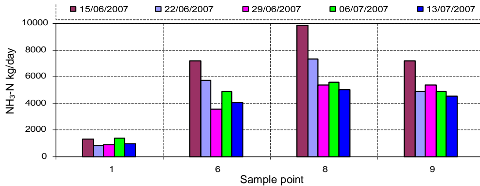
Figure 17. Variation of Ammonia as Nitrogen (NH 3 -N) in kg/day along the Lakhya River.
