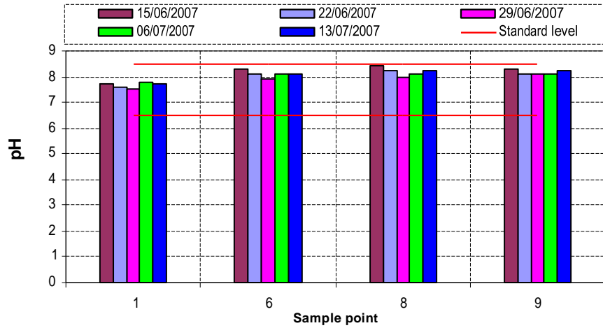
Figure 6. Variation of pH along the Lakhya River.
