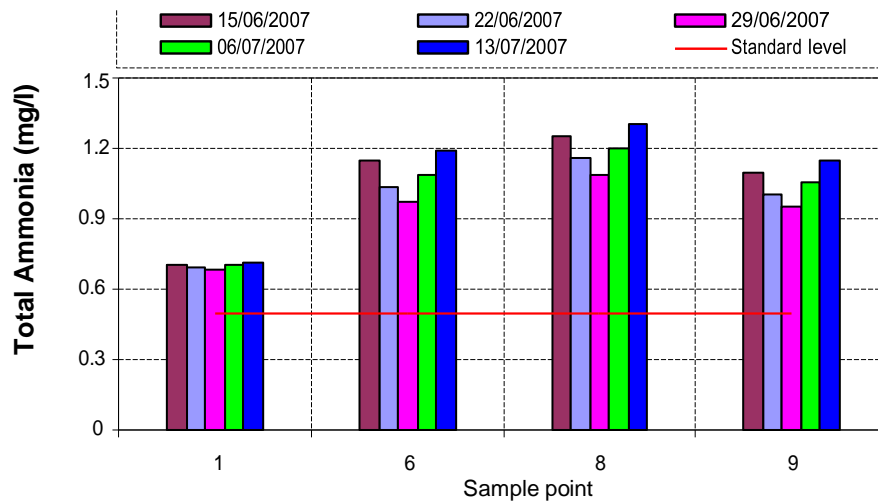
Figure 8. Variation of total Ammonia in mg/l along the Lakhya River.
