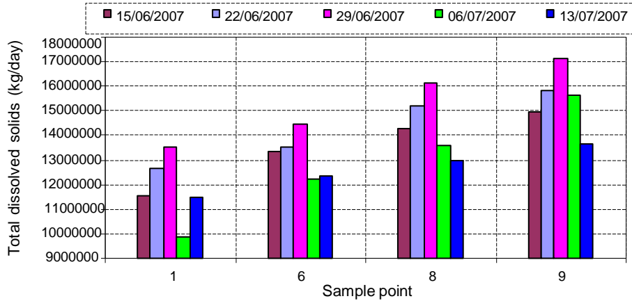
Figure 21. Variation of total dissolved solids in kg/day along the Lakhya River.
