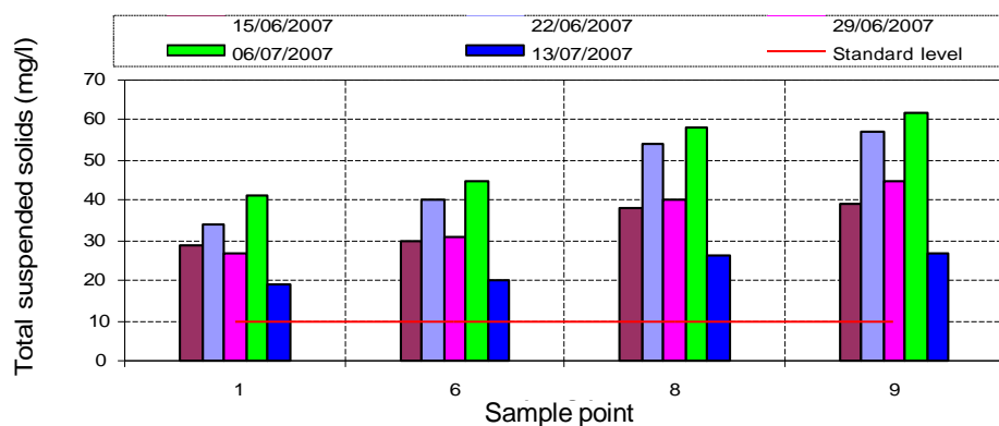
Figure 12. Variations of total suspended solids in mg/l along the Lakhya River.
