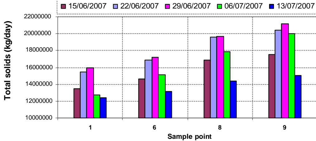
Figure 19. Variation of total solids in kg/day along the Lakhya River.
