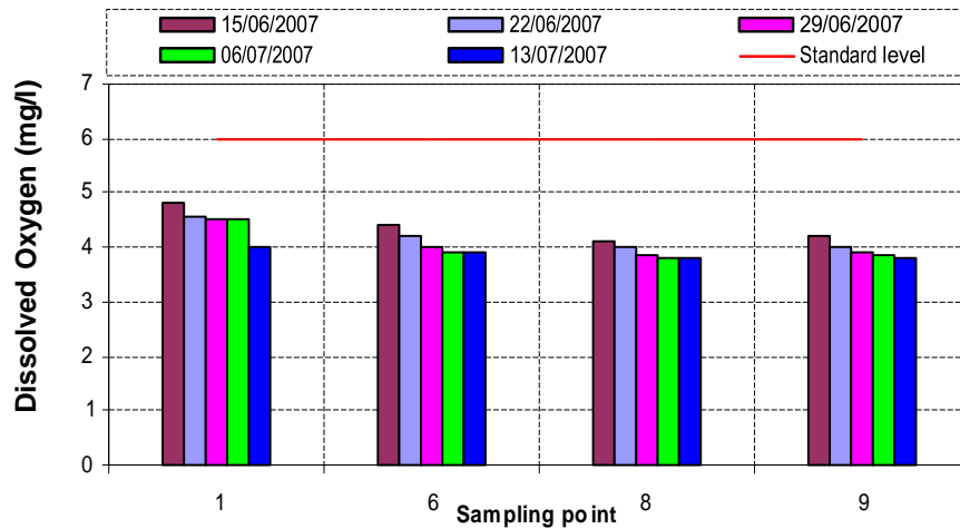
Figure 5. Variation of DO in mg/l along the Lakhya River.
