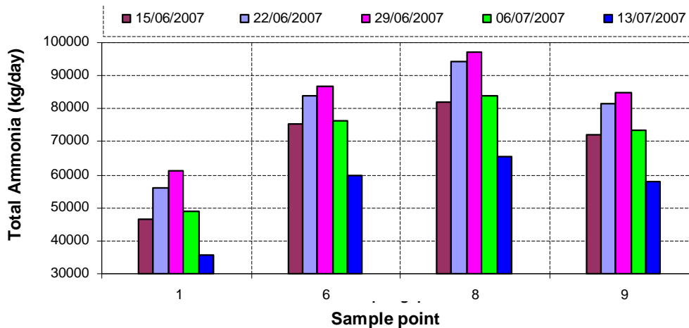
Figure 16. Variation of total ammonia in kg/day along the Lakhya River.
