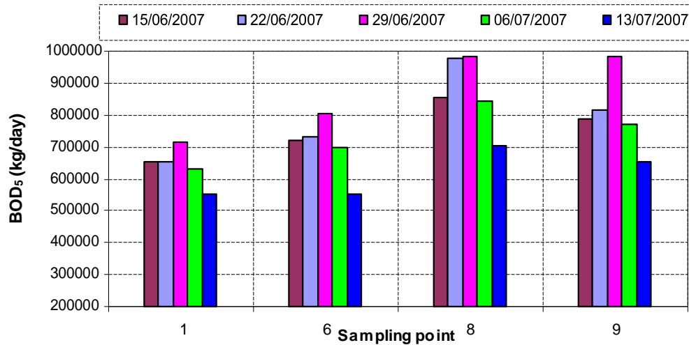
Figure 14. Variation of BOD 5 in kg/day along the Lakhya River.
