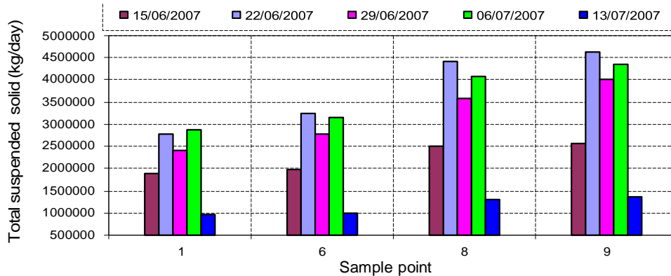
Figure 20. Variation of total suspended solids in kg/day along the Lakhya River.
