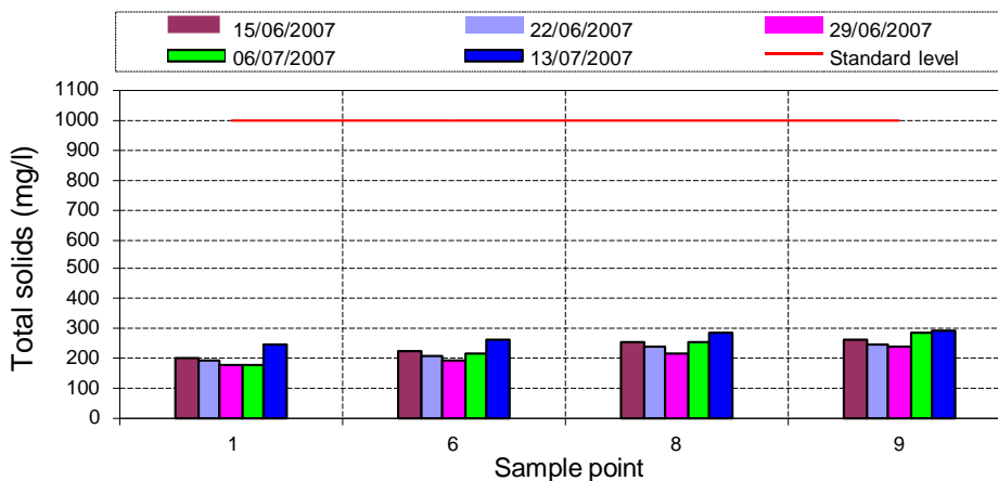
Figure 11. Variations of total solids in mg/l along the Lakhya River.
