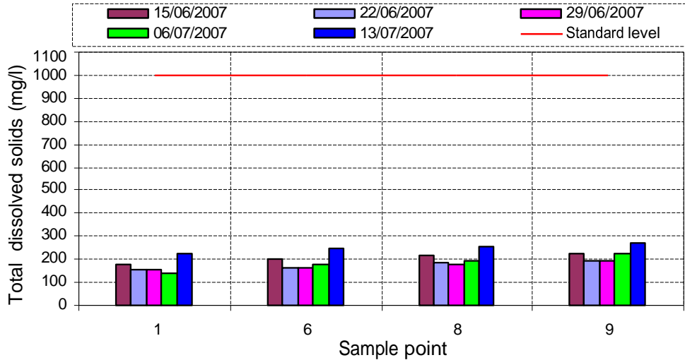
Figure 13. Variation of total dissolved solids in mg/l along the Lakhya River.
