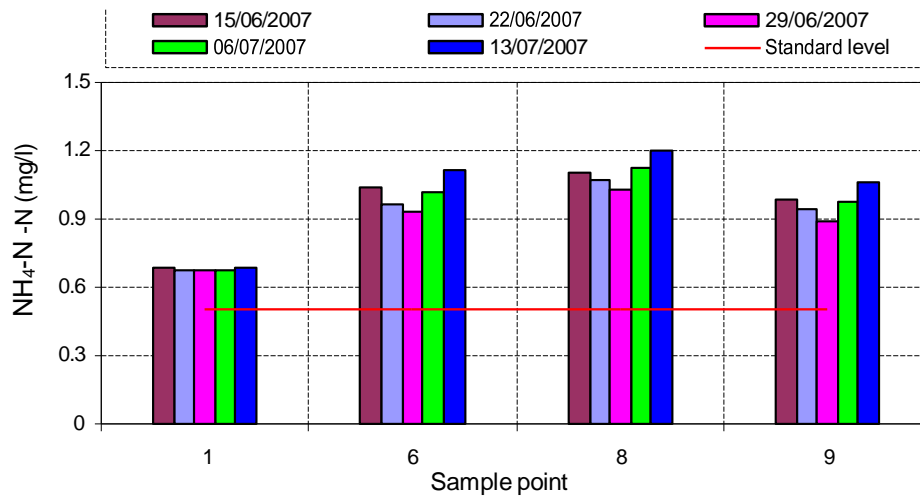
Figure 10. Variation of NH 4 -N in mg/l along the Lakhya River.
