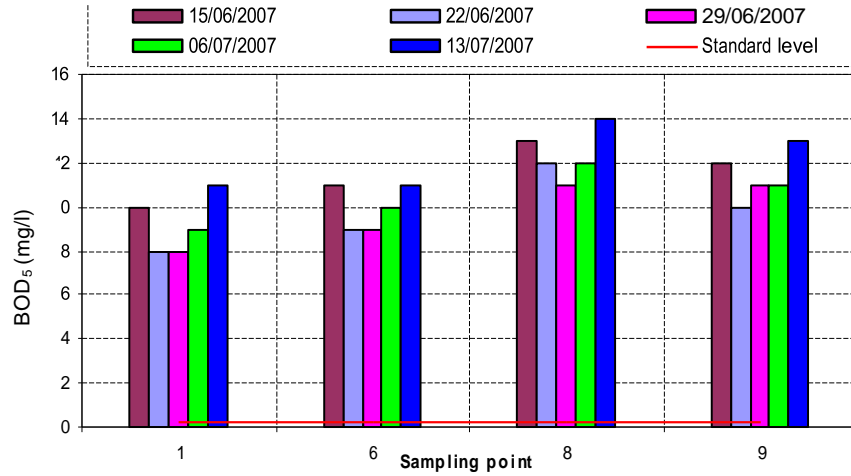
Figure 3. Variation of BOD 5 in mg/l along the Lakhya River.
