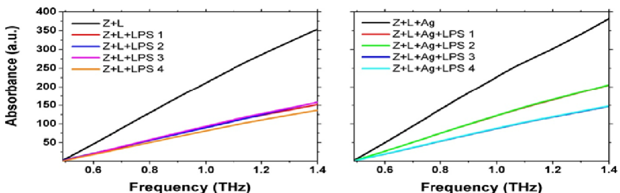
Figure. 2 THz spectra of solutions comprising zein, zein with AgNO 3 (Z+Ag), zein with lecithin (Z+L) and zein with lecithin and AgNO 3 (Z+L+Ag) with LPS molecules normalized to the absorption @ 0.5 THz.
