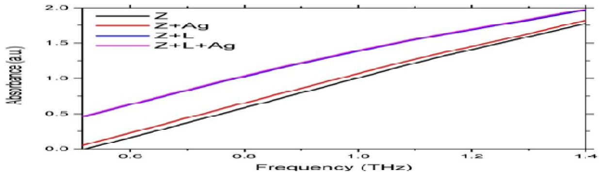
Figure 1 THz spectra of solutions comprising zein, zein with AgNO 3 (Z+Ag), zein with lecithin (Z+L) and zein with lecithin and AgNO 3 (Z+L+Ag)
