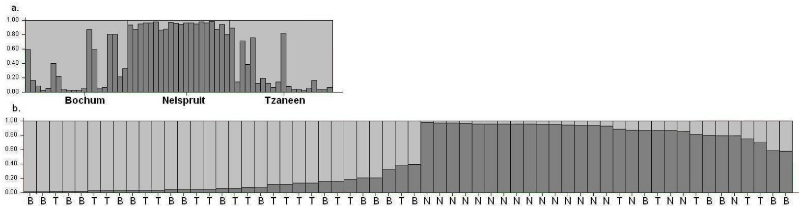
Figure 4. Bar plots (from structure). Each tree is represented by a single vertical line broken into two differently shaded segments, with lengths proportional to membership of each of the two inferred clusters. (a) Three geographic populations in original order. (b) Membership of individuals to two true clusters of marula. Abbreviations used: B=Bochum; N=Nelspruit; T=Tzaneen.
