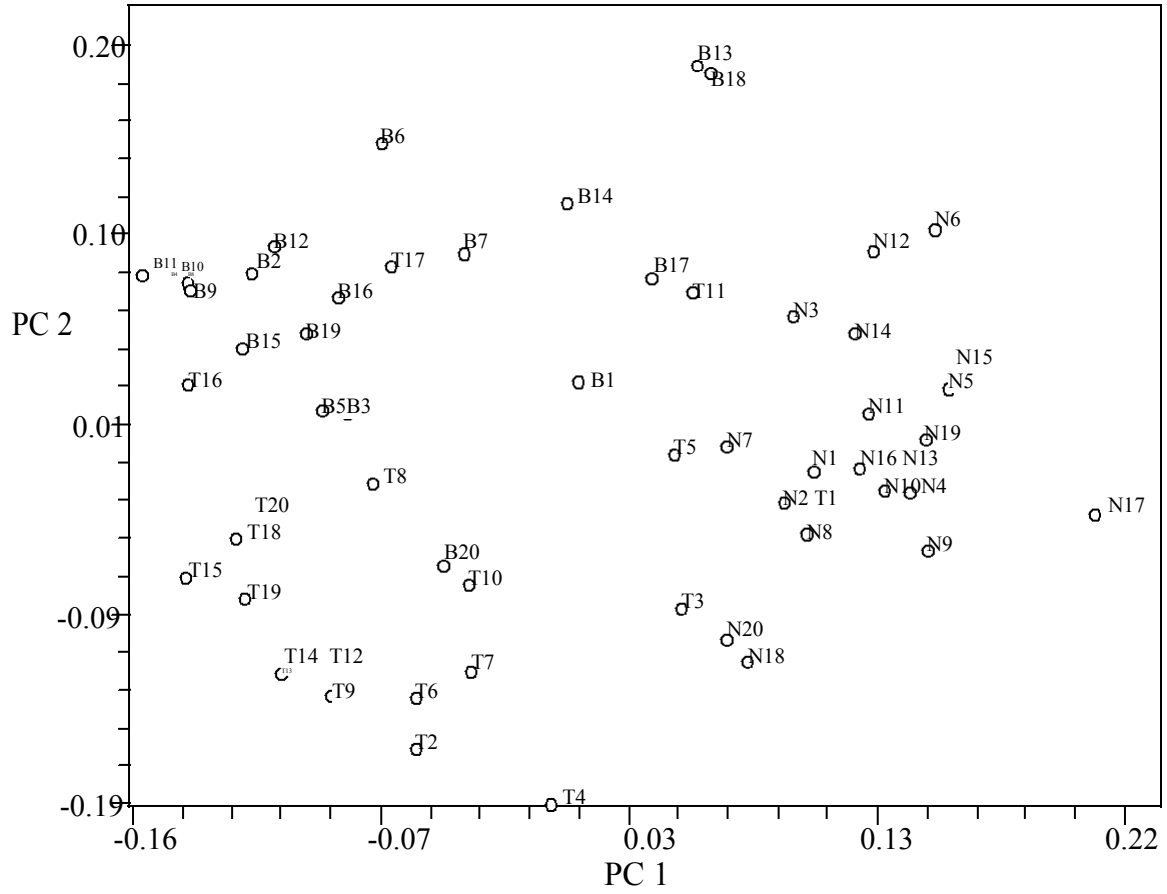
Figure 2. PCO plot showing the dispersal of the natural genotypes in three South African populations, in relation to each other.
