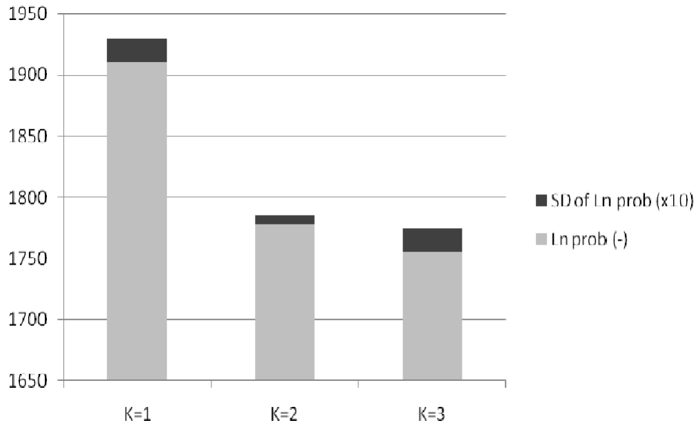
Figure 3. Probability of K=1-3 in three marula populations. Light grey bars show the average -\ln probability for 10 simulations of each value of K; darker areas above bars indicate the standard deviation for 10 simulations.
