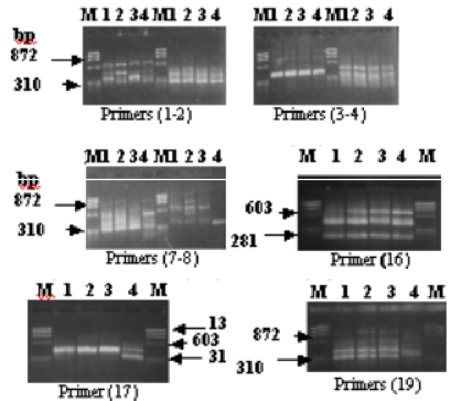
Figure 1. Example of RAPD patterns in four breeds of sheep obtained with different random primers. Lane M: \Phi\text{X174} DNA marker. Lane 1: Baladi, Lane 2: Barki, Lane 3: Rahmani, Lane 4: Saffolk.
