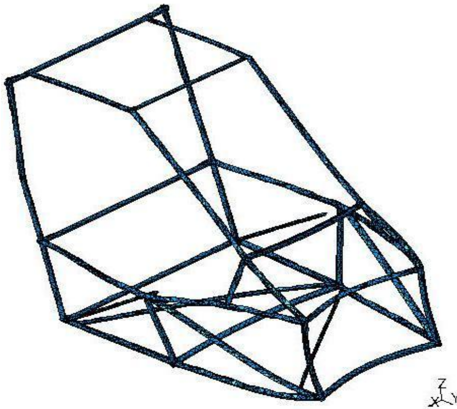
Figure 14. Deformed mesh 3.
