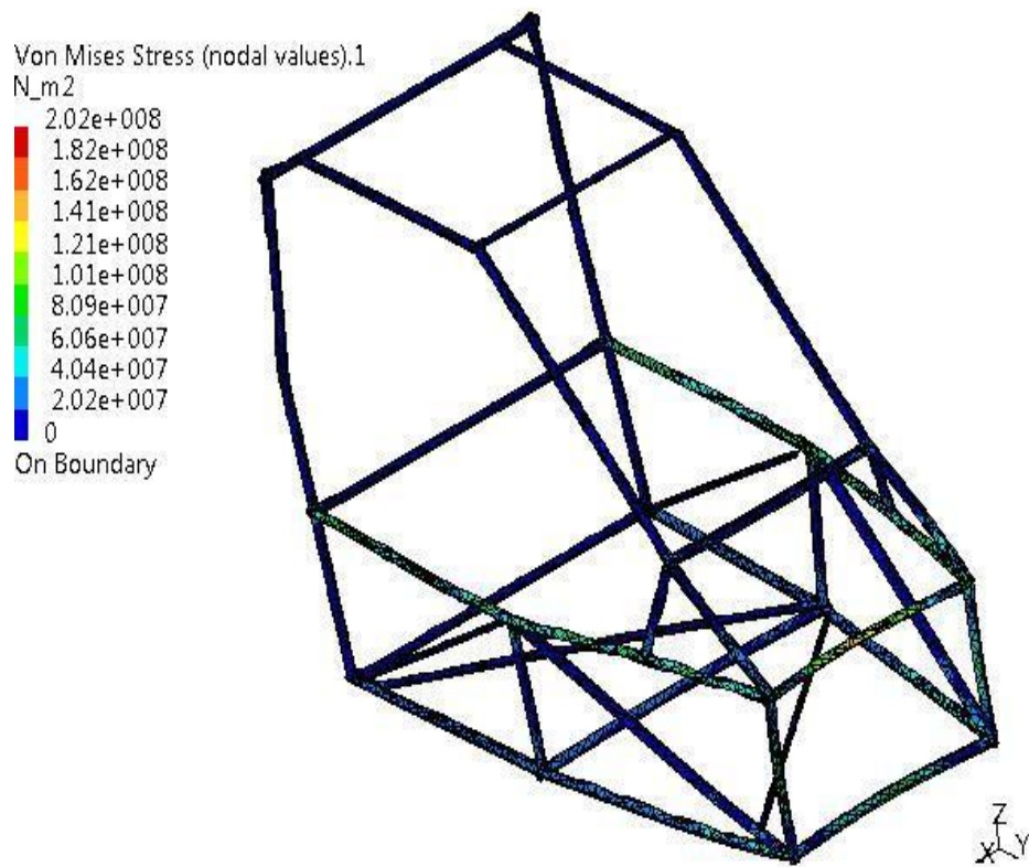
Figure 13. Deformed mesh 2.
