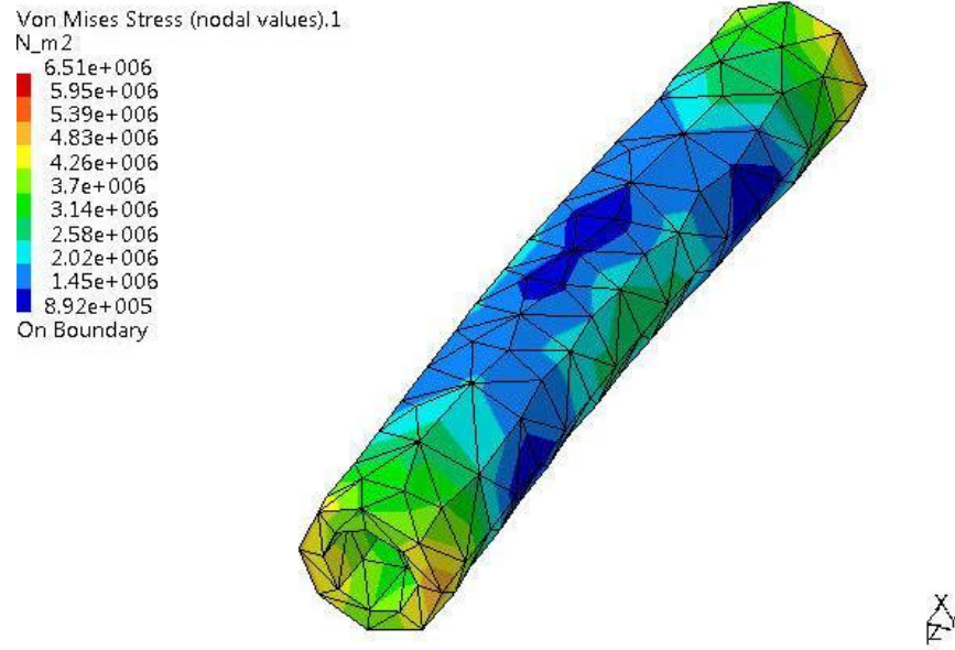
Figure 8. Stress analysis.
