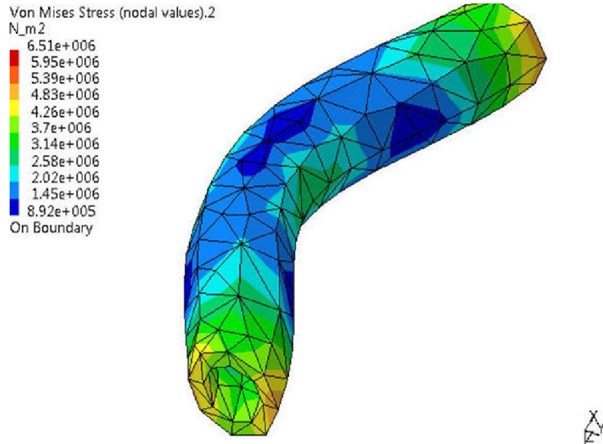
Figure 7. Rod deformation.
