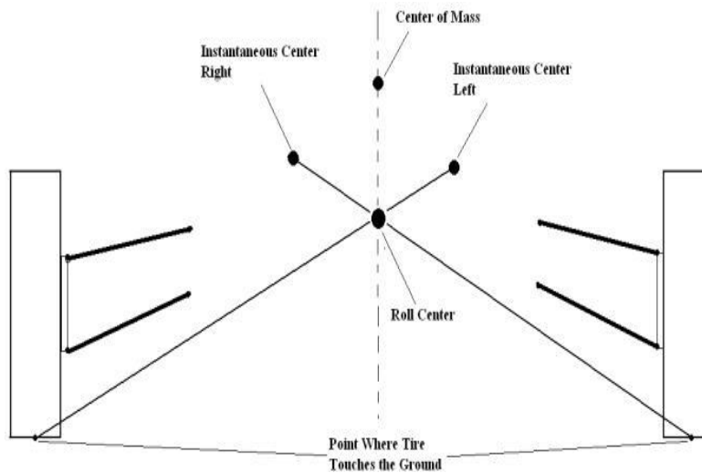
Figure 4. Roll center.
