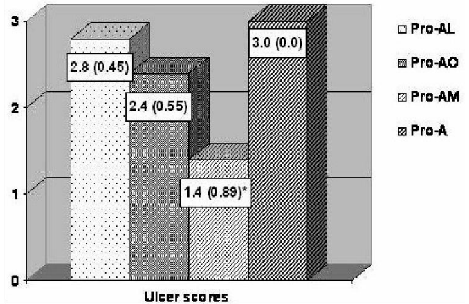
Figure 2. Ulcer scores of different groups in prophylaxis study. Pro-A: aspirin+saline; Pro-AL: aspirin+liquorice; Pro-AM: aspirin+misoprostol; Pro-AO: aspirin+omeprazole; values are expressed as mean (standard deviation); p < 0.05 when compared with controls.
