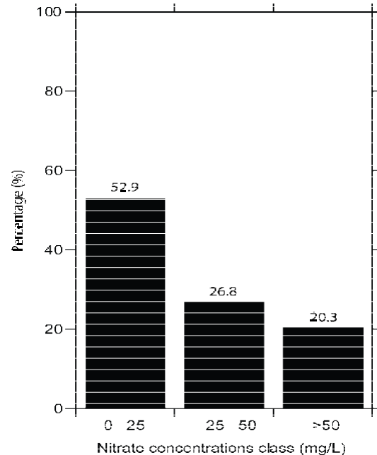
Figure 3. Frequency distribution of NO 3 contents.
