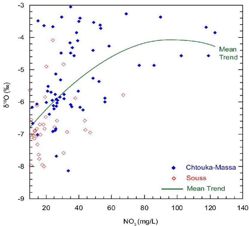
Figure 6. Scatter diagram of \delta^{18}\text{O} vs. \text{NO}_3 in Souss-Massa groundwater. The heavy line represents the mean trend of the \delta^{18}\text{O} - \text{NO}_3 correlation.
