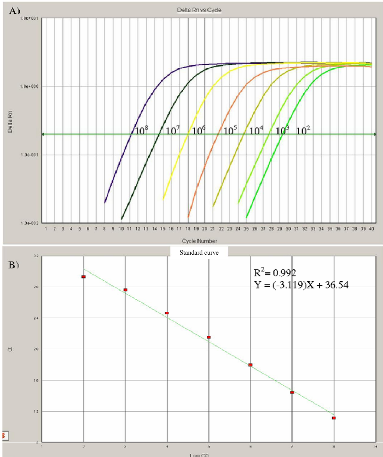
Figure 1. Real- time qPCR standard curve of plasmid containing VP3. A) Dilution series of pVIVO1-VP3 ( 10^8 - 10^2 copies) was amplified using 1 g/ l stock. B) Calibration curve was generated using Ct value versus log copy number (C0). Squares represent Ct values recorded from three independent pVIVO1-VP3 dilutions. The straight line represents linear regression analysis with correlation coefficient ( R^2 ), 0.992.
