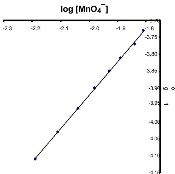
Figure 2. Plot of \log k_1 versus \log [\text{MnO}_4^-] for the redox reaction of malachite green with \text{MnO}_4^- . [\text{MG}^+] = 1.30 \times 10^{-4} \text{ mol dm}^{-3} , [\text{MnO}_4^-] = (6.50 - 16.9) \times 10^{-3} \text{ mol dm}^{-3} , [\text{H}^+] = 5.0 \times 10^{-3} \text{ mol dm}^{-3} , \mu = 0.50 \text{ mol dm}^{-3} , \lambda = 620 \text{ nm} and T = 32.5 \pm 0.5^\circ\text{C} .
