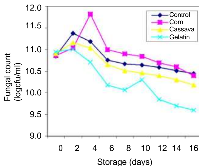
Figure 2. Fungal count (logcfu/ml) of stabilized and unstabilized soy yoghurt samples stored at refrigeration temperature.
