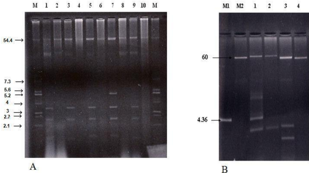
Figure 1. Agarose gel electrophoresis of the plasmidic extract of ESBL and cephalosporinase Salmonella from human in Egypt and their transconjugants. (A) Lane 1-2: Salmonella poona S9 and its transconjugant; Lane 3-4: Salmonella poona S11 and its transconjugant; Lane 5-6: Salmonella poona S12 and its transconjugant; Lane 7-8: Salmonella poona S13 and its transconjugant; Lane 9-10: Salmonella poona S15 and its transconjugant. M: Standard plasmids from E. coli V517 harboring 8 plasmids: 54.4, 7.3, 5.6, 5.2, 4, 3, 2.7 and 2.1 kb. (B) Lane 1- 2 : Salmonella Hadar S4 and its transconjugant; Lane 3-4 Salmonella poona S6 and its transconjugant. M1: RP4 (60kb), M2 : pBR322 (4.36 kb).
