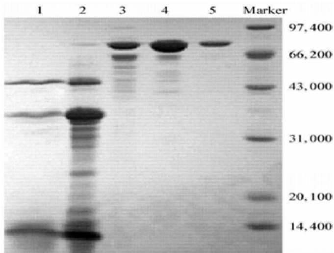
Figure 1. SDS- PAGE. Stacking gel is 3% polyacrylamide in pH 6.8 Tris-HCl buffer. Separation gel is 10% polyacrylamide in pH 8.9 Tris-HCl buffer. All samples were reduced with 2- mercaptoethanol and denatured by a boiling water bath for 5 min before electrophoresis. Protein bands were stained by Coomassie bright blue R- 250. Lane 1: culture supernatant; Lane 2: concentrated fraction from DEAE-Cellulose adsorption; Lane 3: active fraction from DEAE-Cellulose chromatography; Lane 4: active fraction from Phenyl Sepharose chromatography; Lane 5: active fraction from Sephacryl S-100 gel chromatography.
