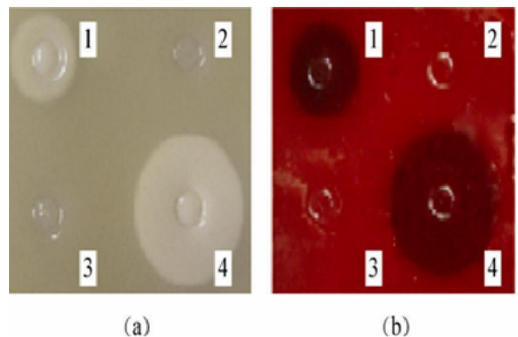
Figure 4. Hemolytic and lecithinase activity assay. 100 ul of samples were added into Oxford cub punched on egg yolk agar or blood agar. (a) is a egg yolk agar (2% egg yolk in 2% agar). (b) is a blood agar (5% washed human erythrocytes in 2% agar). Opal zone in the egg yolk agar indicated the lecithinase activity. Transparent zone in the blood agar indicated the hemolytic activity. The samples were as followings: 1. culture supernatant; 2. purified PLC; 3. physiological saline; 4. control PLC Type 4 from Bacillus cereus (Sigma).
