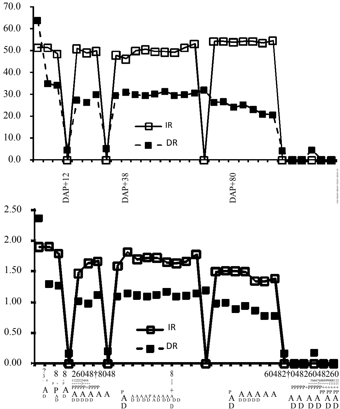
Figure 1. Seasonal transport of suspended solid (upper) and organic matter (lower) into and out of terrace sawah through irrigation (IR) and drainage (DR) water ( \text{kg ha}^{-1} ) within a rice cropping season.
