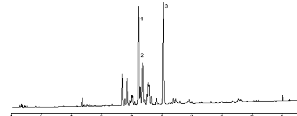
Figure 5. HPLC chromatogram of ethanol extract of Piper guineense . 1 = (Piperanine, 2 = \alpha , - Dihydrowasanine, 3 = N- isobutyl- (E, E)-2, 4-decadienamide).
