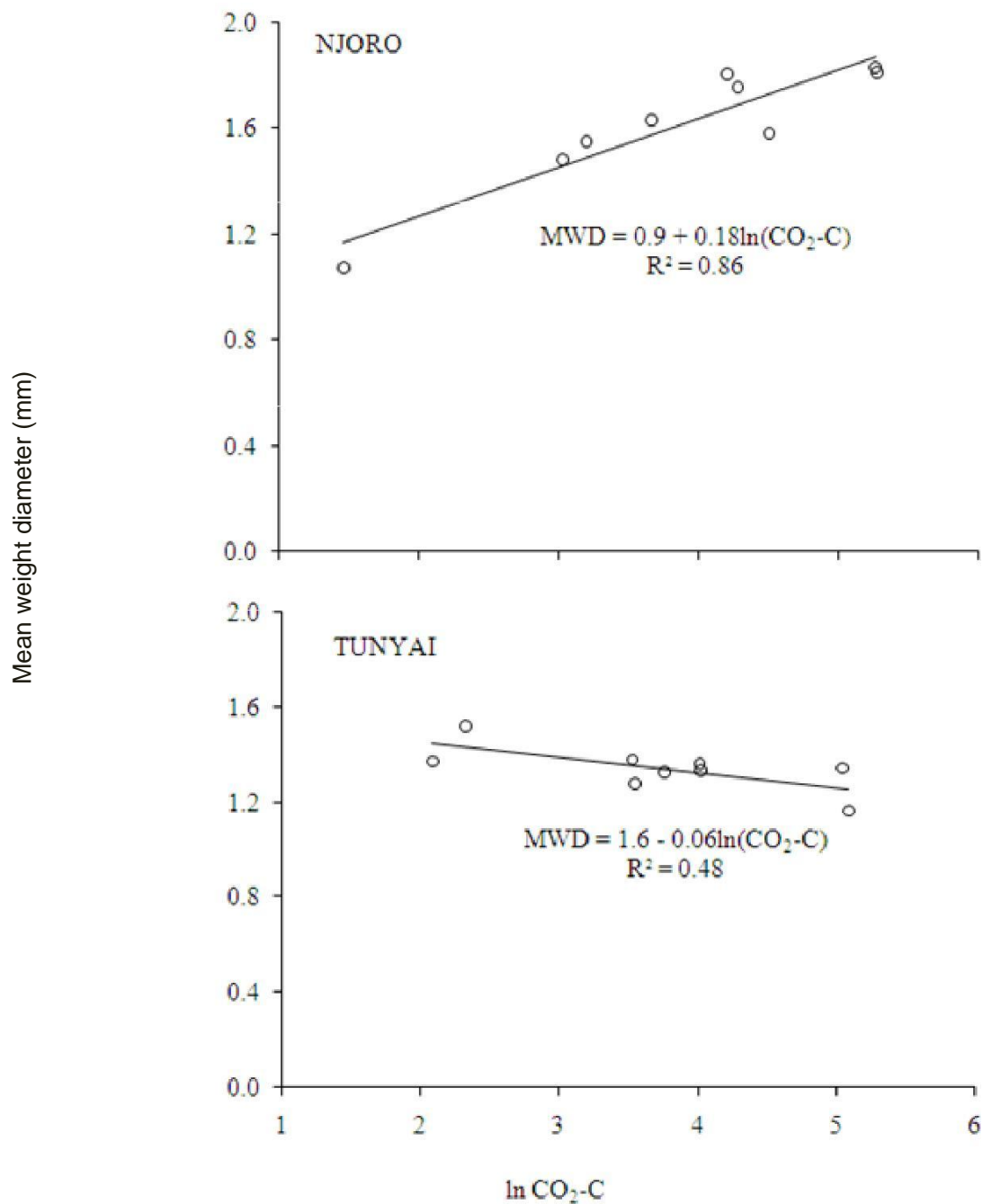
Figure 3. Mean weight diameter (MWD) as a function of CO 2 -C evolution for the soils from the two locations.
