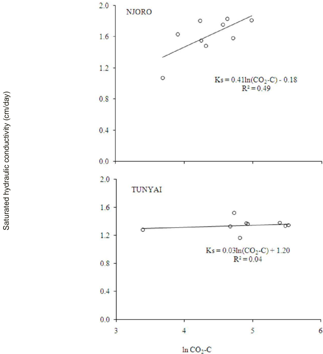
Figure 4. Saturated hydraulic conductivity (Ksat) as a function of CO 2 -C evolution for the soils from the two locations.
