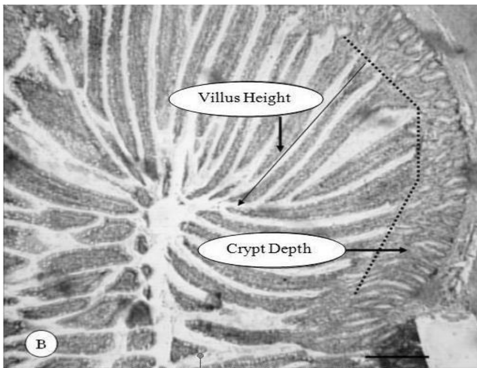
Figure 2. Bird from the treated group with \beta -mannanase (700 g/ton). Section of a duodenal tissue of broiler chicken. Scale bar represents 500 \mu\text{m} .
