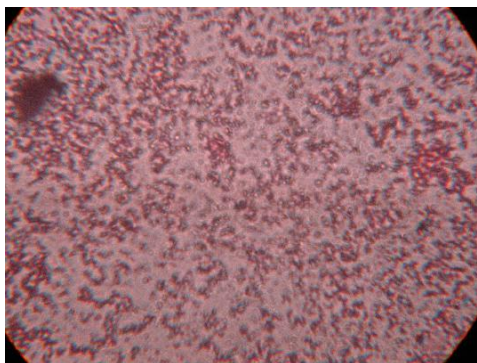
Figure 1. Microscopical view of chitinase producing bacterium Micrococcus sp. AG84.
