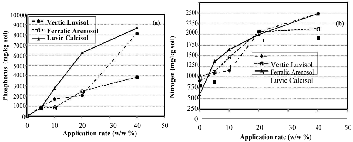
Figure 4. Available nutrient concentrations in selected soils types at different application rates: (a) Phosphorus and (b) Nitrogen (significant at p < 0.05 ).
