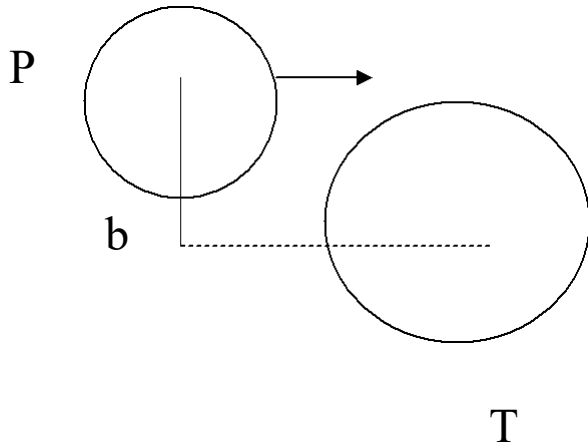
Figure (1-a) An interaction projectile P incident to a Target T at a given impact parameter b
