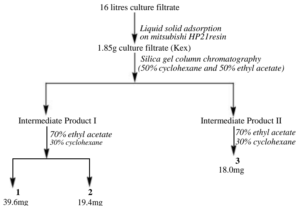
Figure 1. Purification scheme for compounds 1, 2 and 3 from Stereum species (JO5289).
