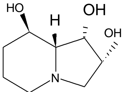
Figure 1. Structure of swainsonine.
