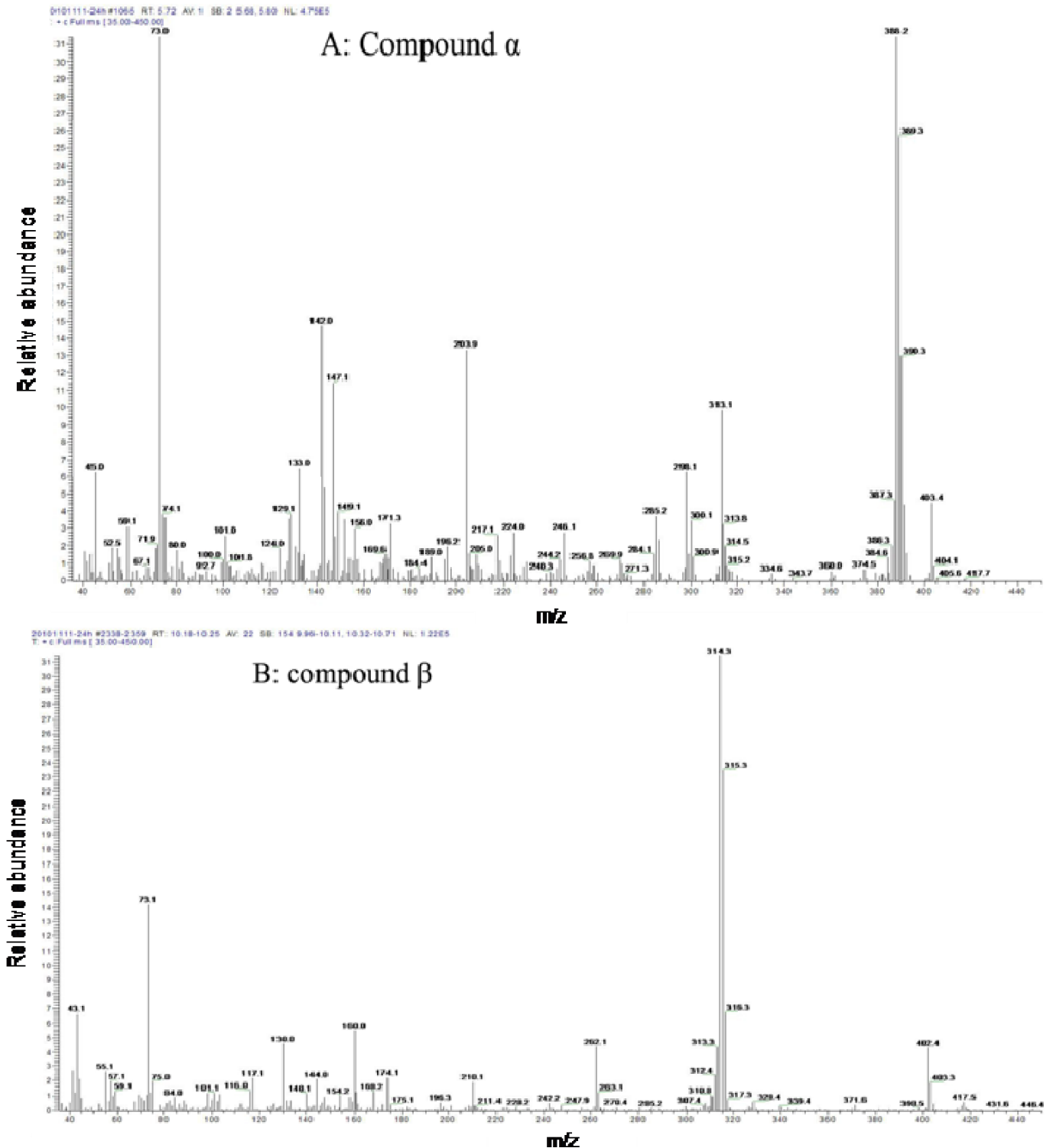
Figure 6. The mass spectrometry of metabolites for SW degradation by 5 types of transformants detected by Trace DSQ. Intermediate metabolite: (A) compound and (B) compound .
