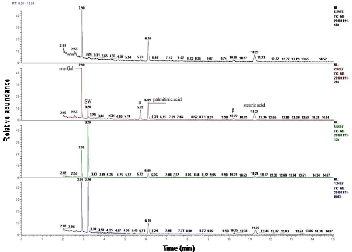
Figure 5. The gas chromatography of 1 \text{ g l}^{-1} SW degradation by 5 transformants with Trace GC.
