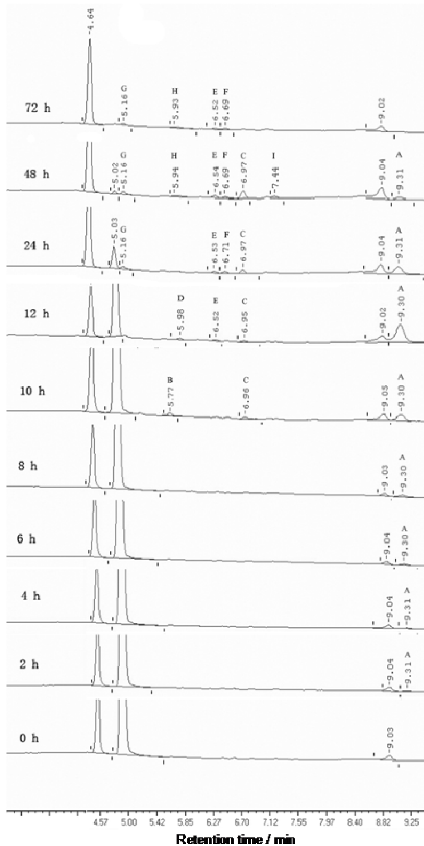
Figure 4. The gas chromatography of 1 \text{ g l}^{-1} SW degradation by the mixture of 5
