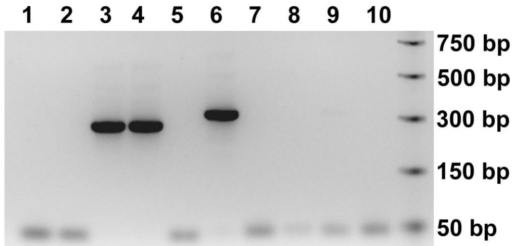
Figure 2 SCC mec characterization by PCR. SCC mec type III PCR is shown in lanes 1-5. SCC mec type V PCR is shown in lanes 6-10. Lane 1 and 6, isolate 59A; lane 2 and 7, isolate 72B; lane 3 and 8, isolate 94; lane 4 and 9, isolate 95C; lane 5 and 10, no template control. Molecular weight PCR marker (Promega) is shown.
