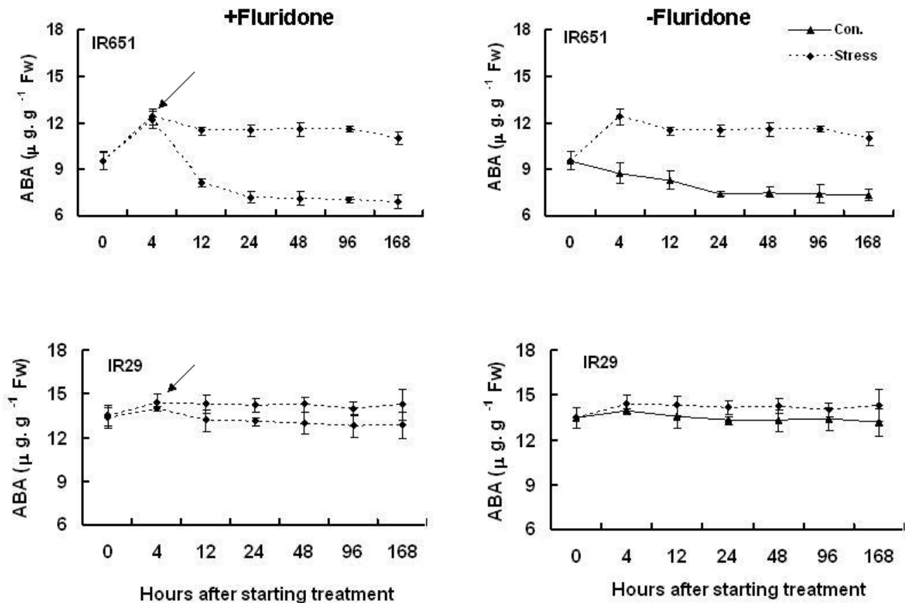
Figure 3. ABA measured on the youngest fully expanded leaf of two rice cultivars during the seedling stage under control and salt stress of 12 dsm -1 . The data are mean values of three replications with three measurements per replication, and vertical bars represent ±SE of the mean (n=3) where these exceed the size of the symbol. The values on the x-axis represent of hours after the start of salt stress treatment of 21-day-old seedlings. The arrows indicate the spraying of Fluridone.
